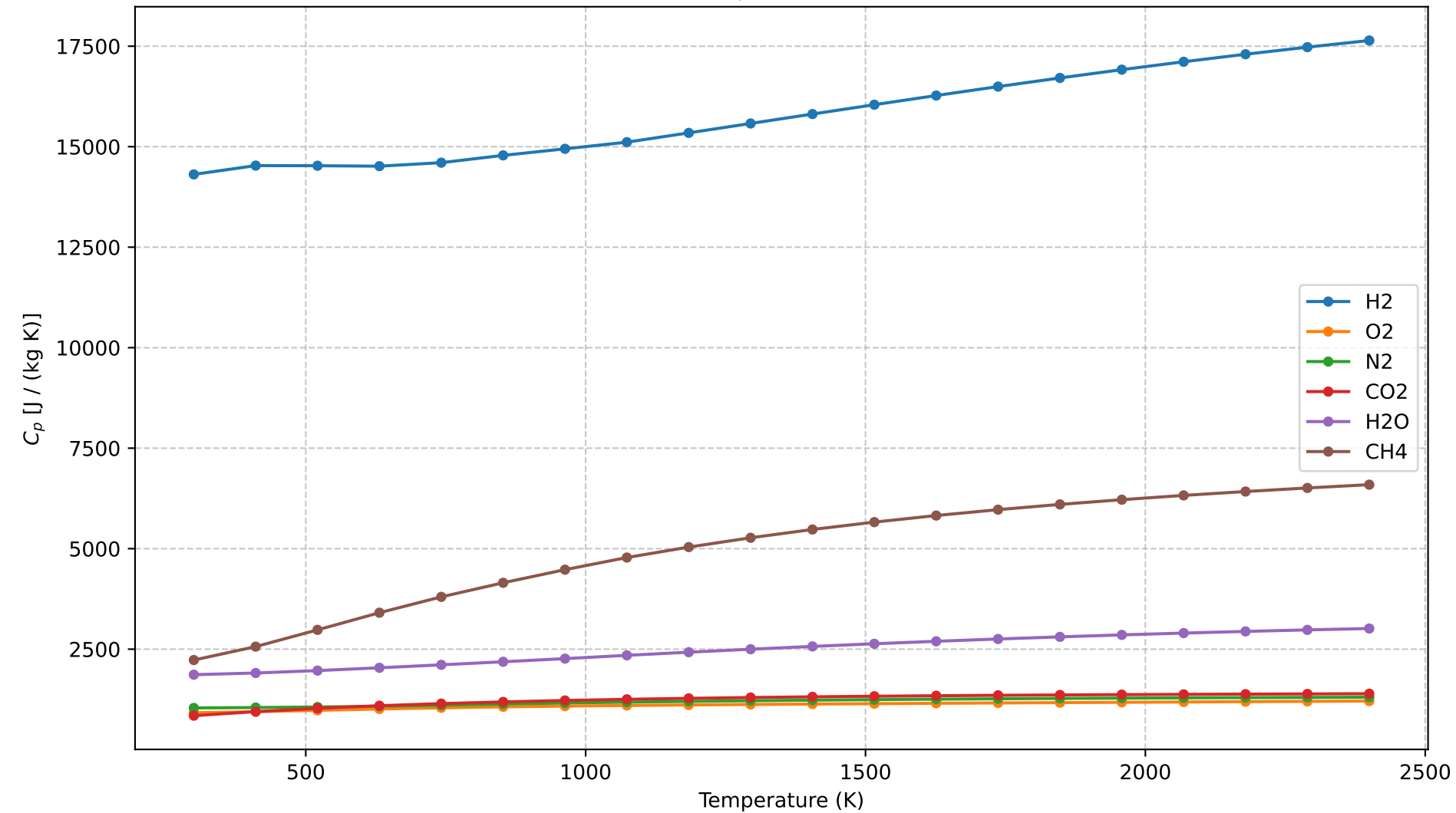
Variation of Specific Heat ( C_p ) with Temperature Using Cantera
